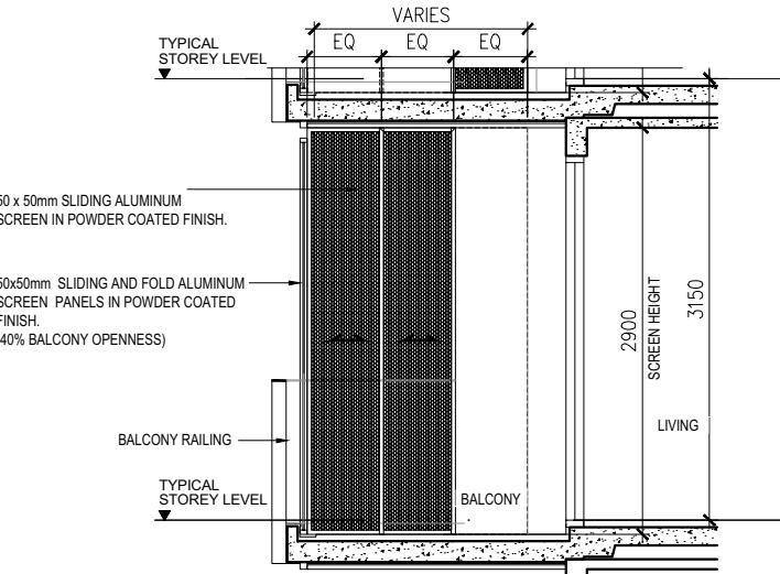
BALCONY / PES SCREEN - SECTION A-A (Internal View)
